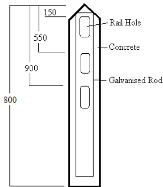
Side View EFP1800-03PT
