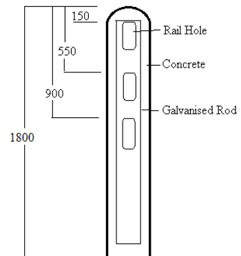
Side View EFP1800-03RT
