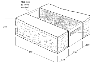
Stack Pillar Mail Box Block with inserts GSP-M
