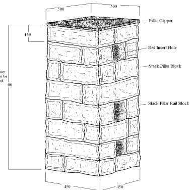
Stack Pillar Rail 3 Way Block GSP-3W
